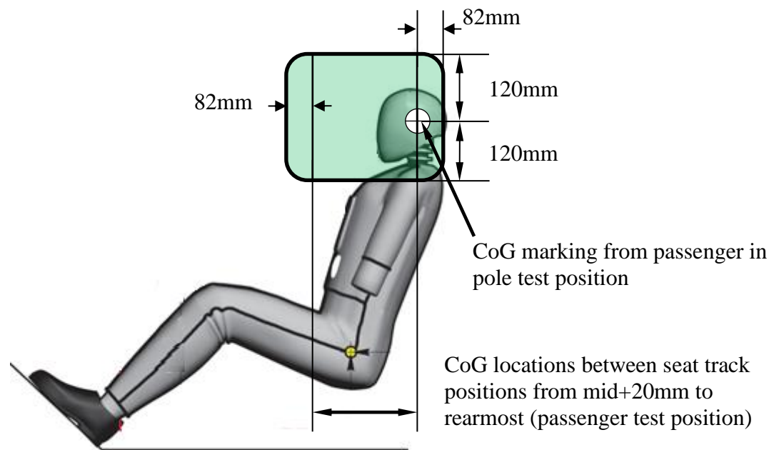
Figure 6: Protection zone
